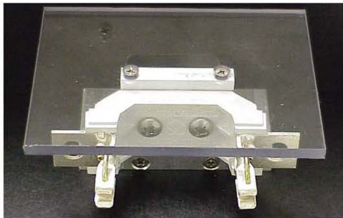
Front close-up of UUT Mating Connector
