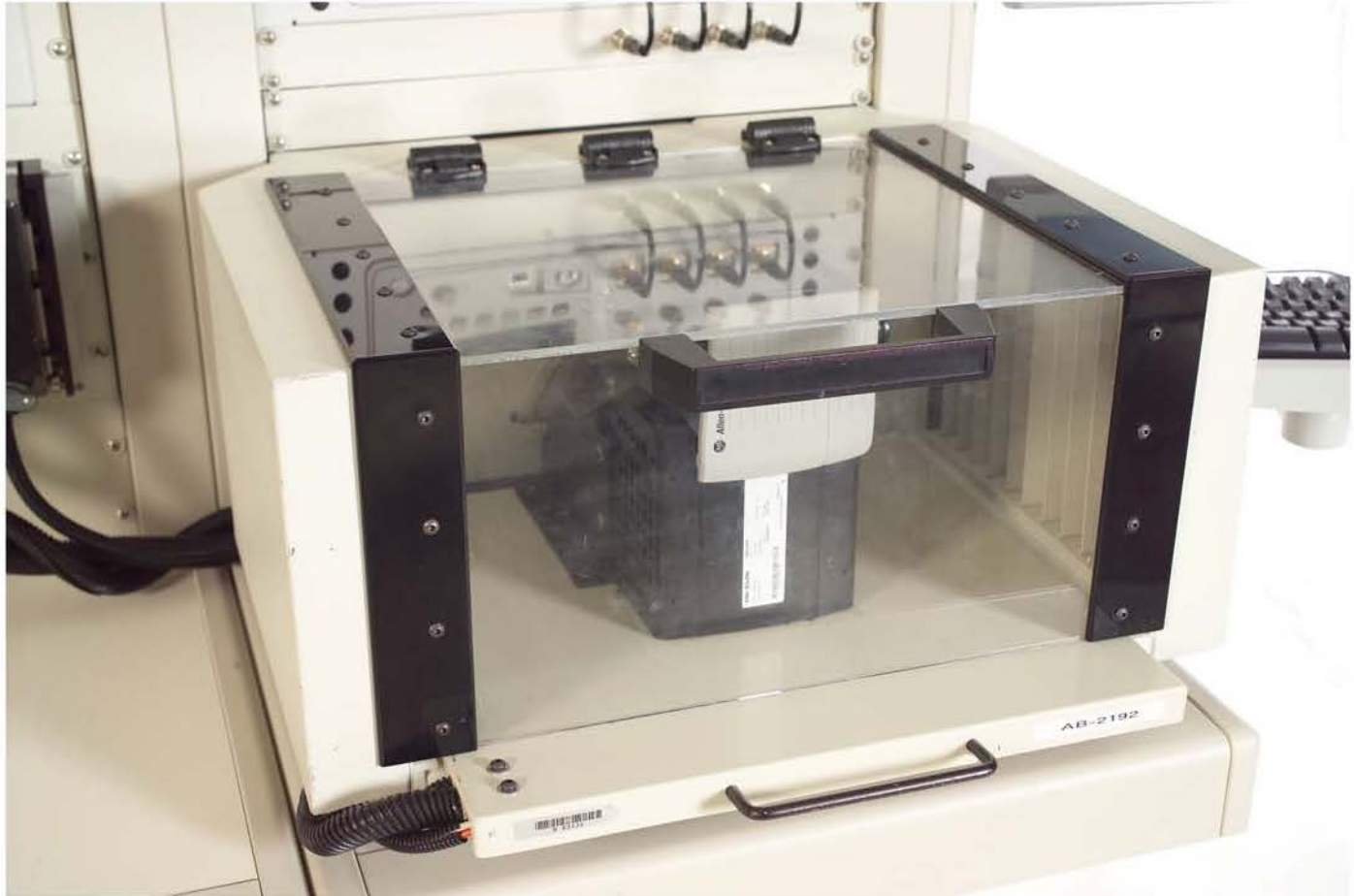
Test Fixture with a UUT Installed
