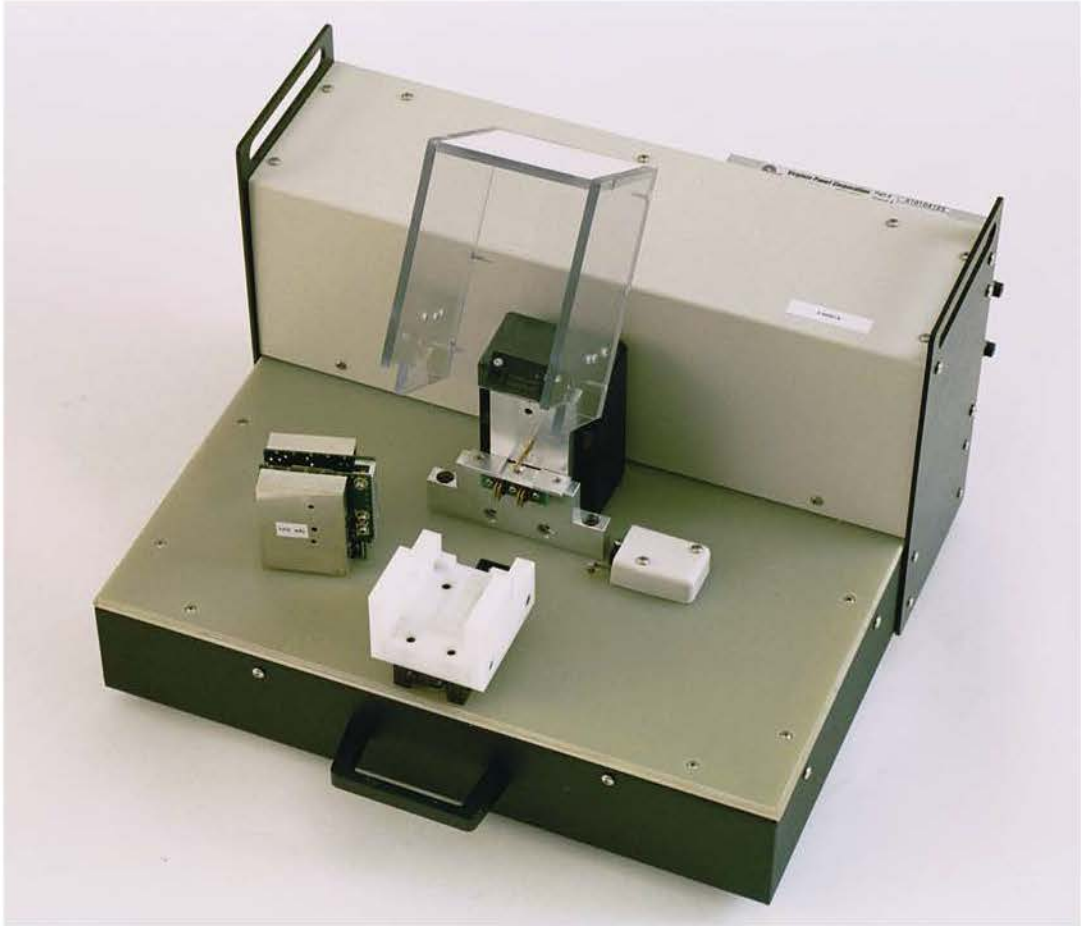
Front view of Test Fixture with UUT
