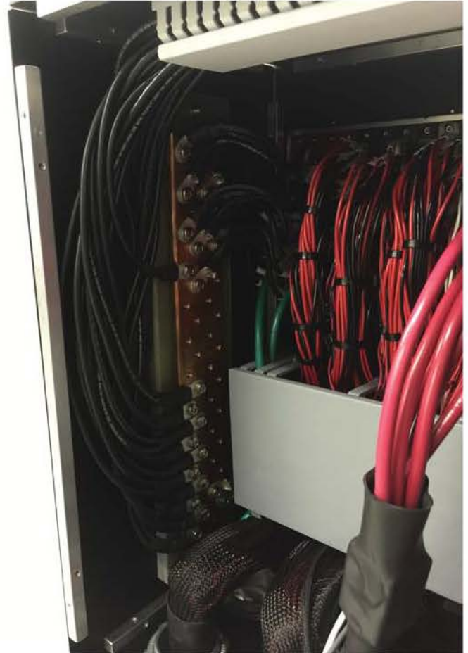
Inside ITA/Cable Harness with Bus Bars
