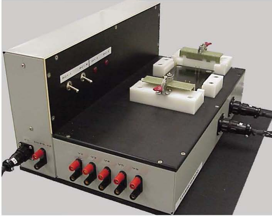
Side view of Test Fixture
