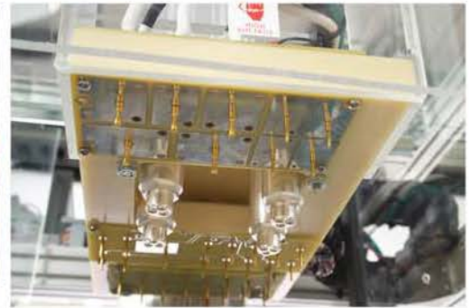
Close-Up 250Amp Pogo-Pins
